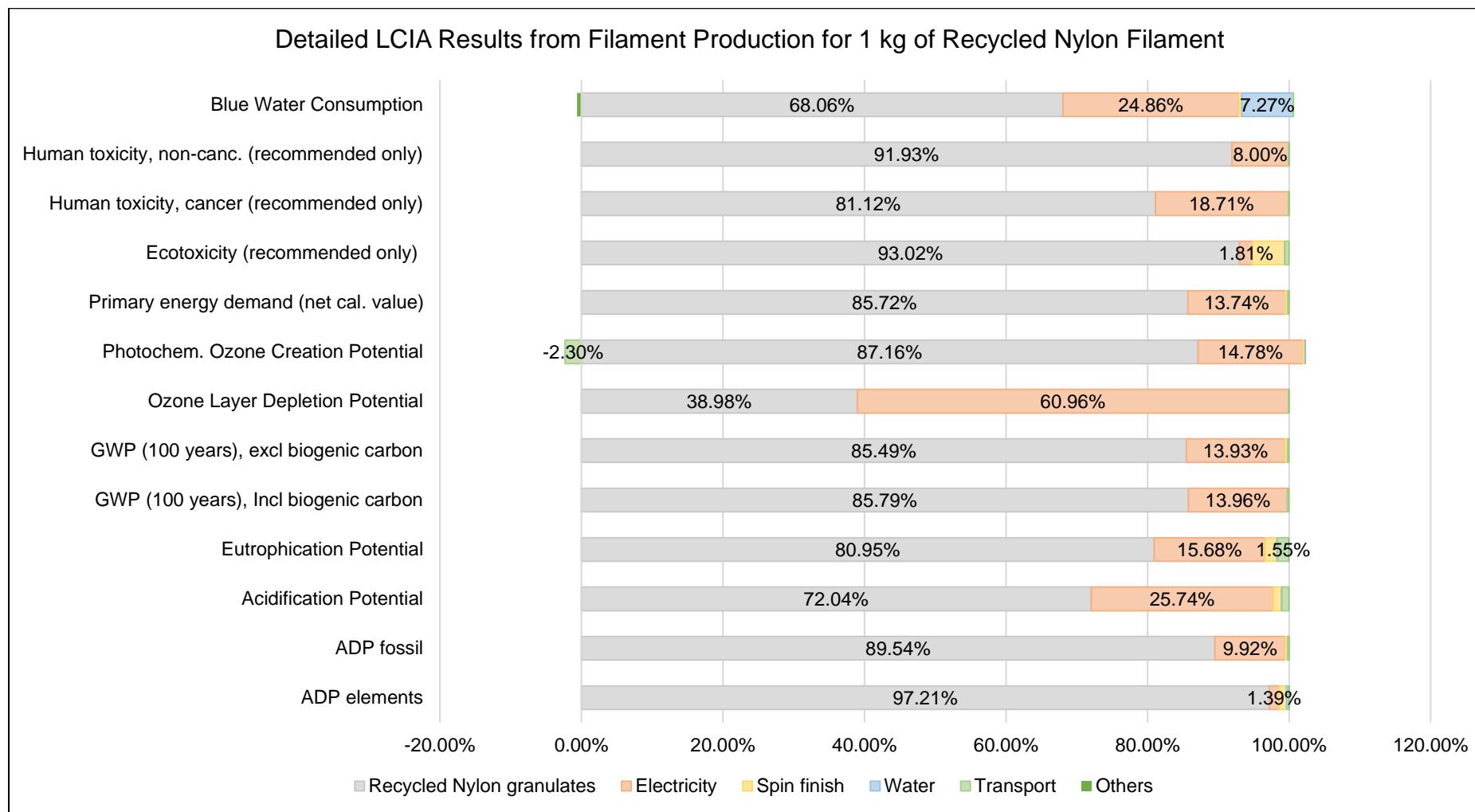
Figure 4-1 Detailed LCIA Results from Filament Production Process for Recycled Nylon Filament Product
