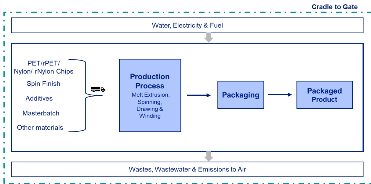
Figure 2-1 System boundary for Recycled Nylon Filament product
