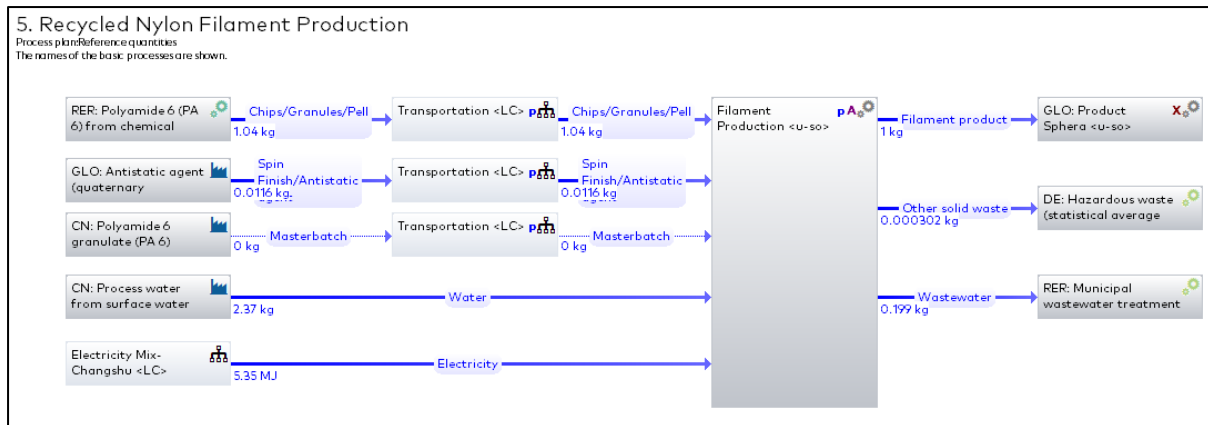
Figure 3-2 LCA FE model snapshot of Recycled Nylon Filament Production from Filament manufacturing
